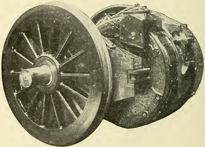
Fig. 264. Grand Trunk Locomotive Motor Mounted on Driving Wheels
